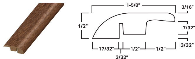
Reducer
